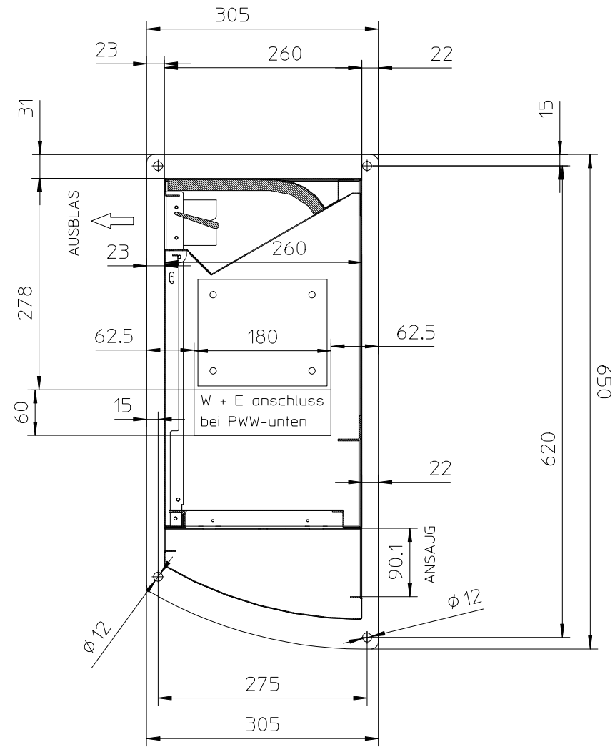
Section 3-3 SCALE 1:5
